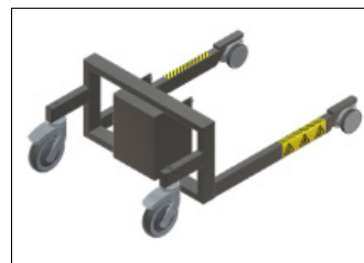
STANDARD Rear wheel with brake Leg length: 500 mm
